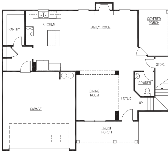
Main Level
