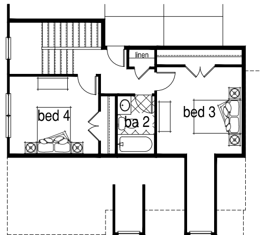
Optional Bed 3/ Bed 4 / Bath 2 ILO Bonus Room 2
