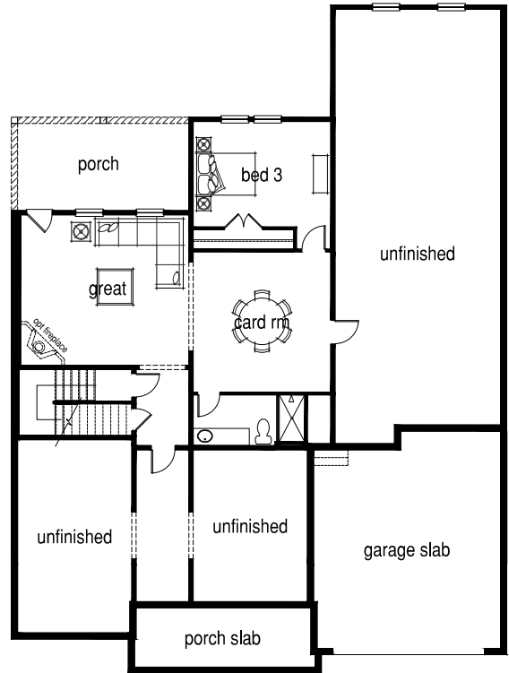
Opt. Finished Basement #2
