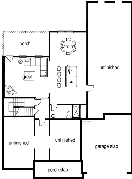
Opt. Finished Basement #1
