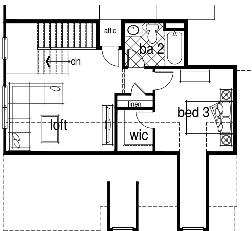
Opt. Bed 3/ Bath 2 with Loft ILO Bonus Room 2 (At 6:12 Roof Pitch)
