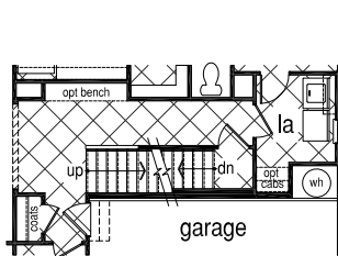
Stair to Opt Basement with Second Floor
