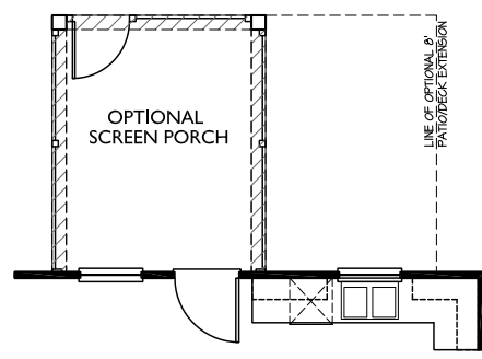
opt screen porch
