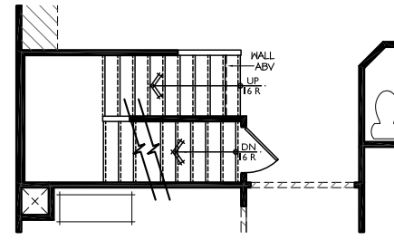
stairs at opt basement
